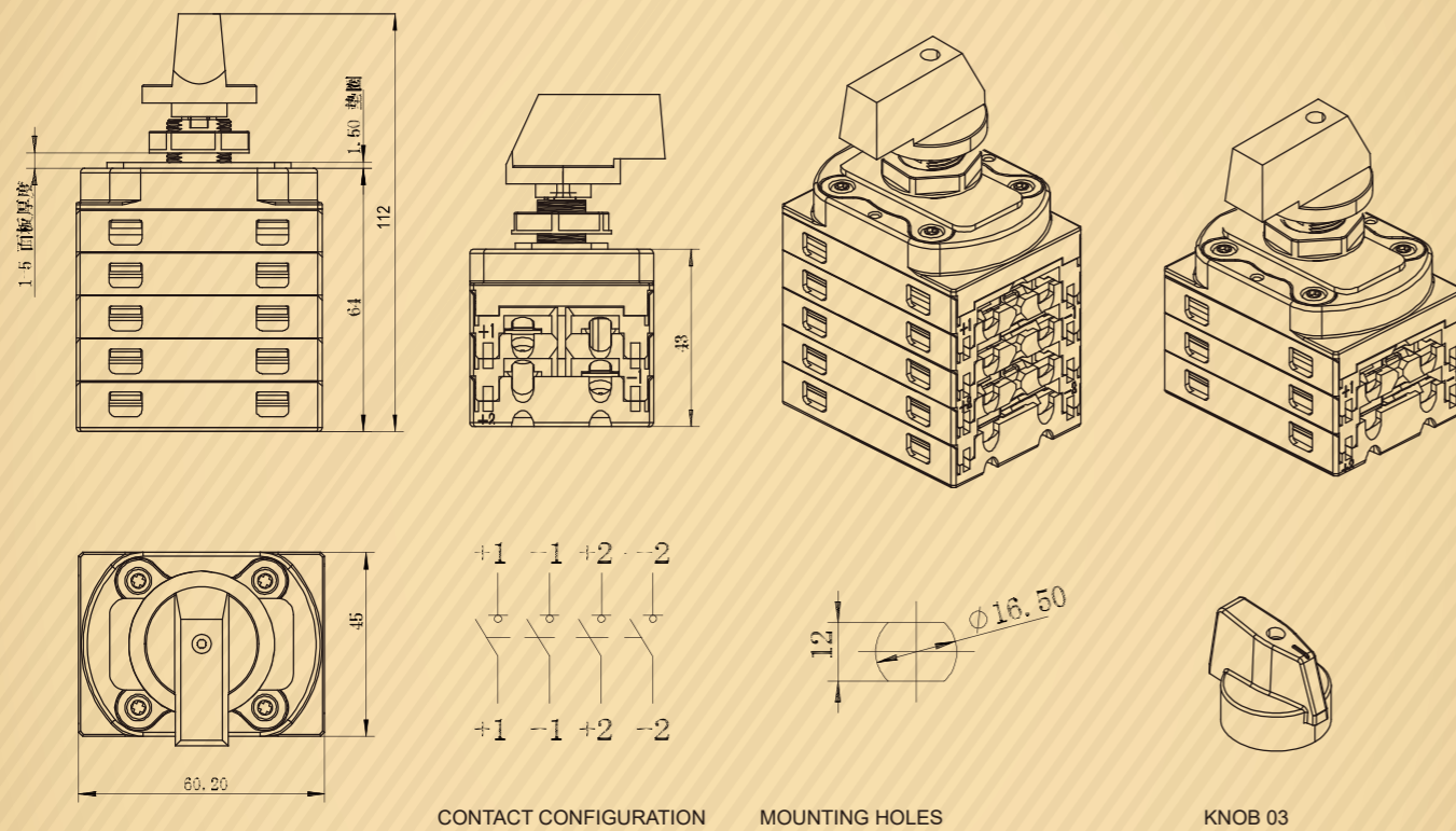
CONTACT CONFIGURATION
